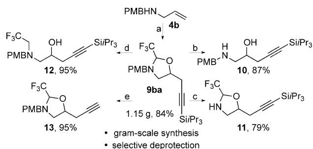
Scheme 6. Scale-up and orthogonal deprotections. Reaction conditions: a) 4.5 equiv 5a , 1.3 equiv 3a , 4 mol % 6 , 6 mol % 7a , 1.3 equiv \text{Cs}_2\text{CO}_3 in toluene at 60 °C; b) p -toluenesulfonic acid, THF/MeOH (9:1), 60 °C; c) DDQ, \text{CH}_2\text{Cl}_2/\text{H}_2\text{O} (24:1); d) DIBAL-H, toluene, –78 to –25 °C; e) TBAF, THF. DIBAL-H = diisobutylaluminum hydride, DDQ = 2,3-dichloro-5,6-dicyano-1,4-benzoquinone, PMB = para -methoxybenzyl, TBAF = tetra- n -butylammonium fluoride, THF = tetrahydrofuran.
