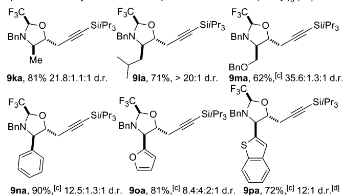
c) Methylallyl amines ( R^3 \neq H ): [a] 1.5 equiv 3 and 6 mol % XantPhos ( 7b )
